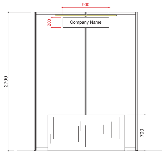
Elevation Plan
