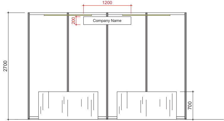
Elevation Plan
