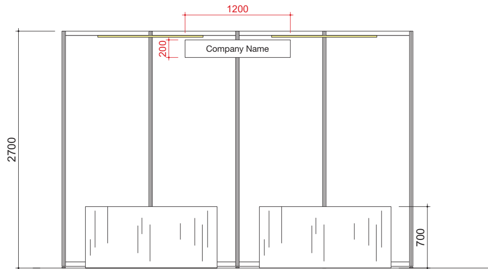
Elevation Plan
