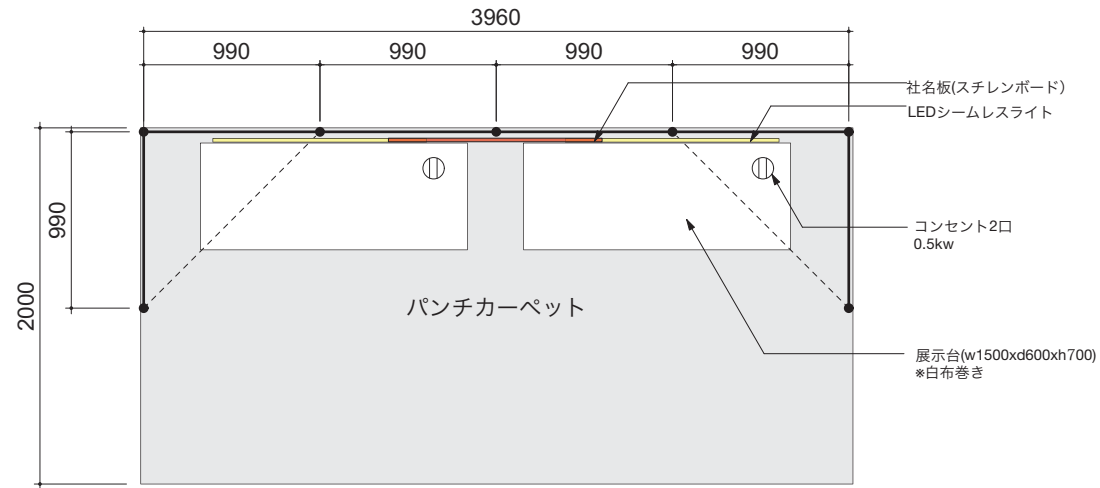
Floor Plan
