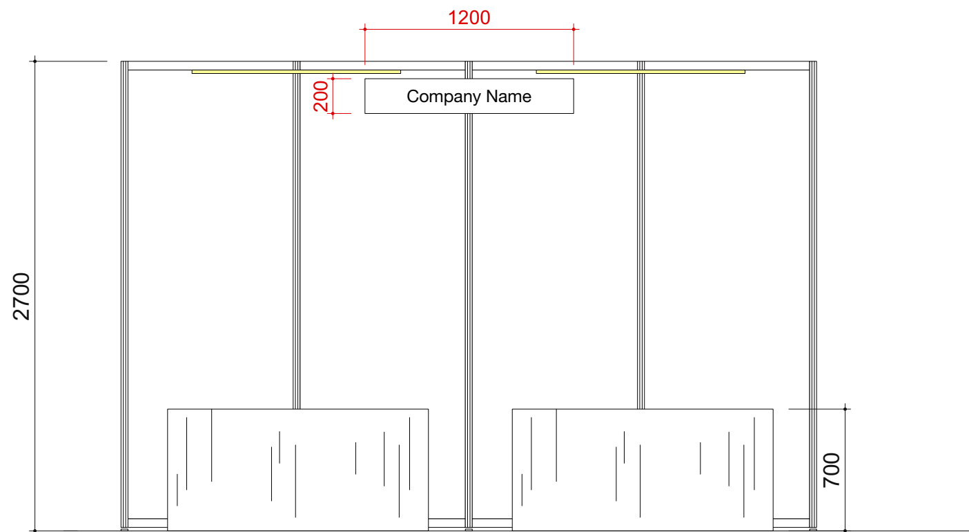
Elevation Plan
