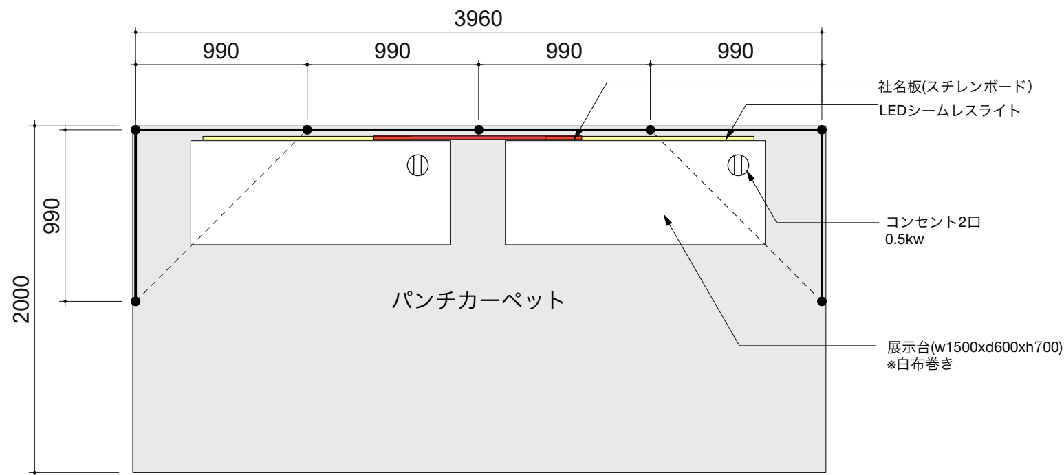
Floor Plan
